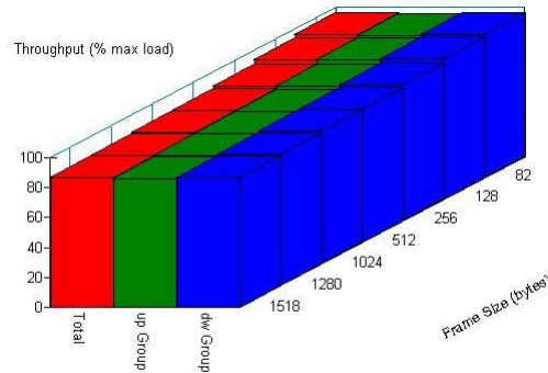
Throughput vs Frame Size
